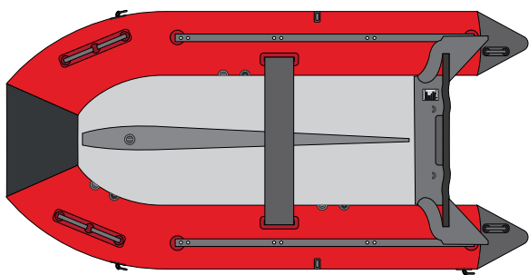
DS320 Inflatable - Technical Drawing.
